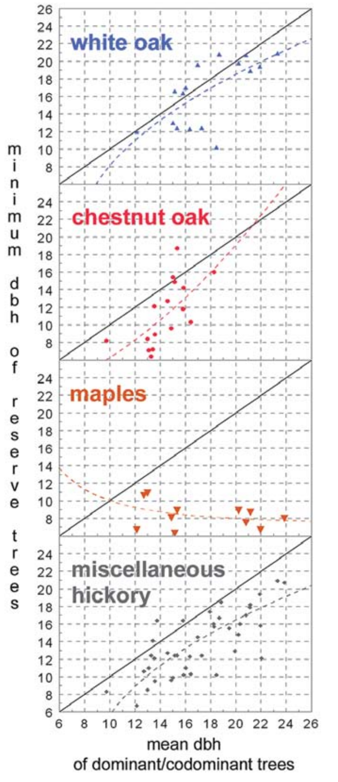
Figure 4. Minimum average dbh for reserve trees for species groups based on the average dbh of dominant and co-dominant trees in each stand for seven tracts on the Cumberland Plateau in eastern Kentucky. The diagonal line shows a 1:1 relationship.
